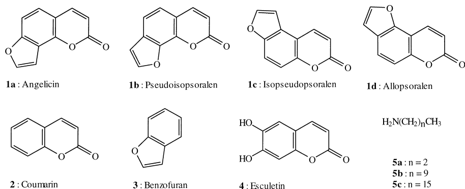
Figure 1. Structure of some coumarins and other simple building blocks used in this study.
