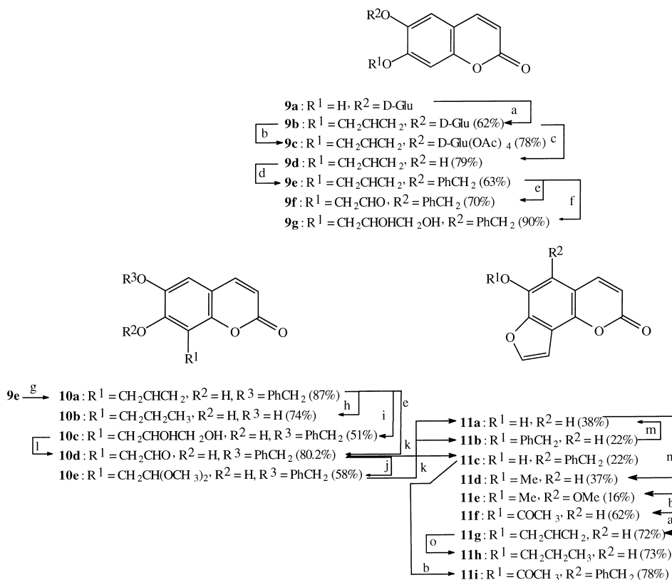
Scheme 2. Synthesis of compounds 9a–g , 10a–e , and 11a–i . (a) allyl bromide, K 2 CO 3 /DMF; (b) acetic anhydride, DMAP, NEt 3 /CH 2 Cl 2 ; (c) H 2 SO 4 /H 2 O; (d) benzyl bromide, K 2 CO 3 , NaI/DMF; (e) NaIO 4 , OsO 4 /THF, MeOH, H 2 O; (f) NMO, OsO 4 /THF, MeOH, H 2 O; (g) 215–225°C, 1 mm Hg; (h) H 2 , Pd–C/MeOH; (i) NMO, OsO 4 /acetone, EtOAc, H 2 O; (j) 10-camphorsulfonic acid/MeOH; (k) p -toluenesulfonic acid/C 6 H 6 (total yield 82%); (l) NaIO 4 /THF, MeOH, H 2 O; (m) H 2 , Pd(OH) 2 /EtOAc, MeOH; (n) (CH 3 ) 2 SO 4 , K 2 CO 3 /MeOH (total yield 53%); (o) H 2 , Pd–C/EtOAc, MeOH.
