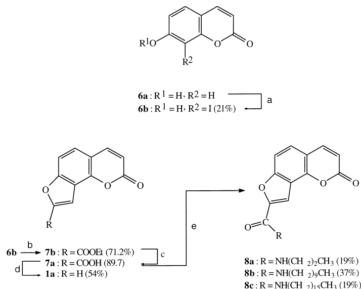
Scheme 1. Synthesis of compounds 1a , 7a,b and 8a–c . (a) \text{I}_2, \text{KI}/\text{H}_2\text{O} ; (b) \text{CH}\equiv\text{CCOOEt}, \text{Cu}_2\text{O}/\text{DMF}, 110^\circ\text{C} ; (c) \text{NaOH}/\text{H}_2\text{O} ; (d) \text{Cu}/\text{quinoline} ; (e) I. \text{SOCl}_2 ; II. \text{H}_2\text{NR}/\text{THF}, \text{DMAP} .
